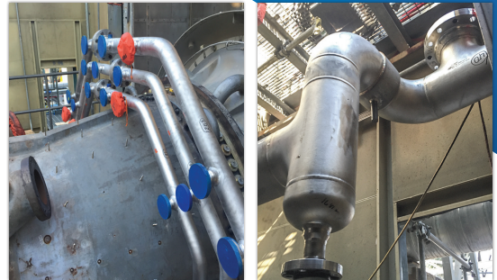
Piping Fabrication & Install
