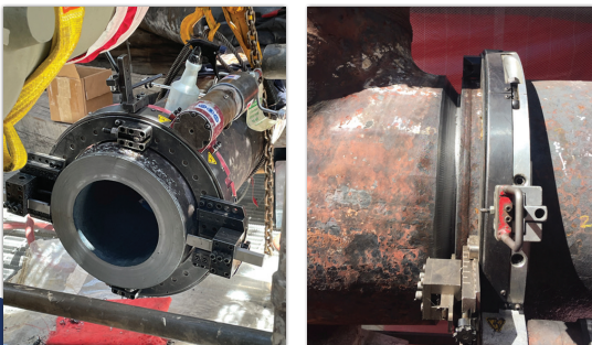
Precision Machine Weld Joints
